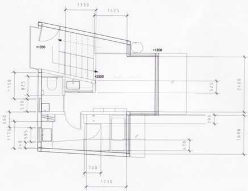
upper level GA Plan
