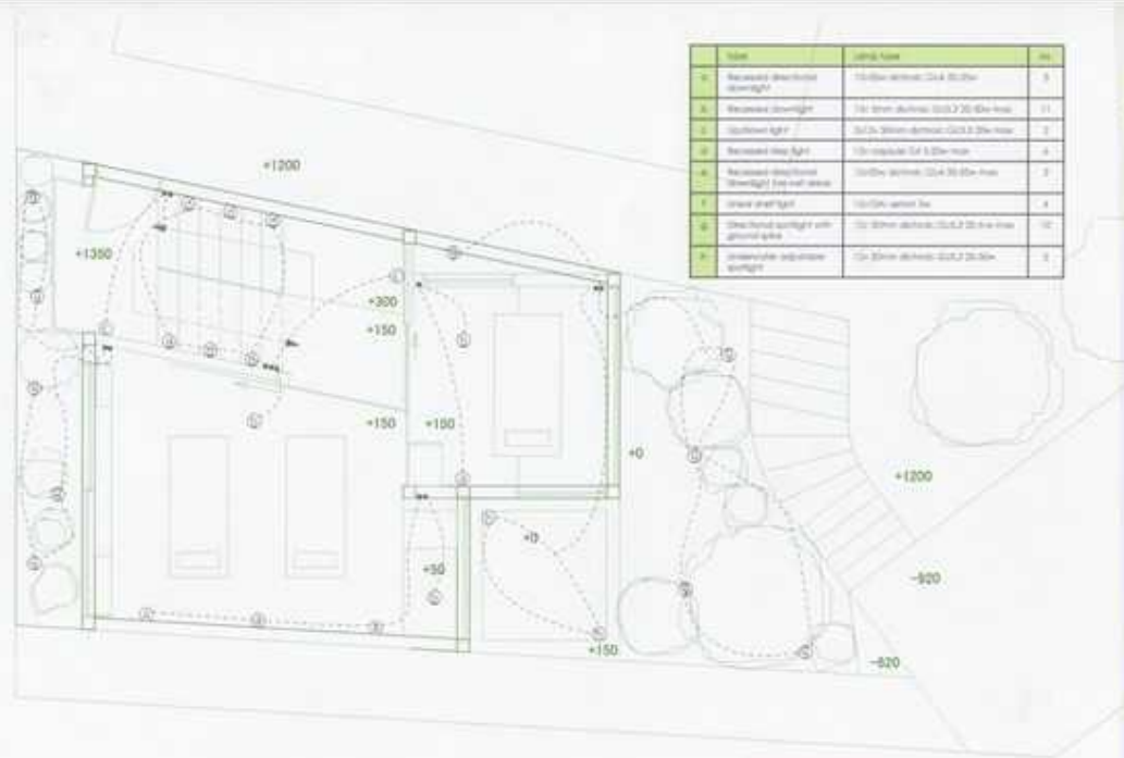
lower level Lighting Plan
